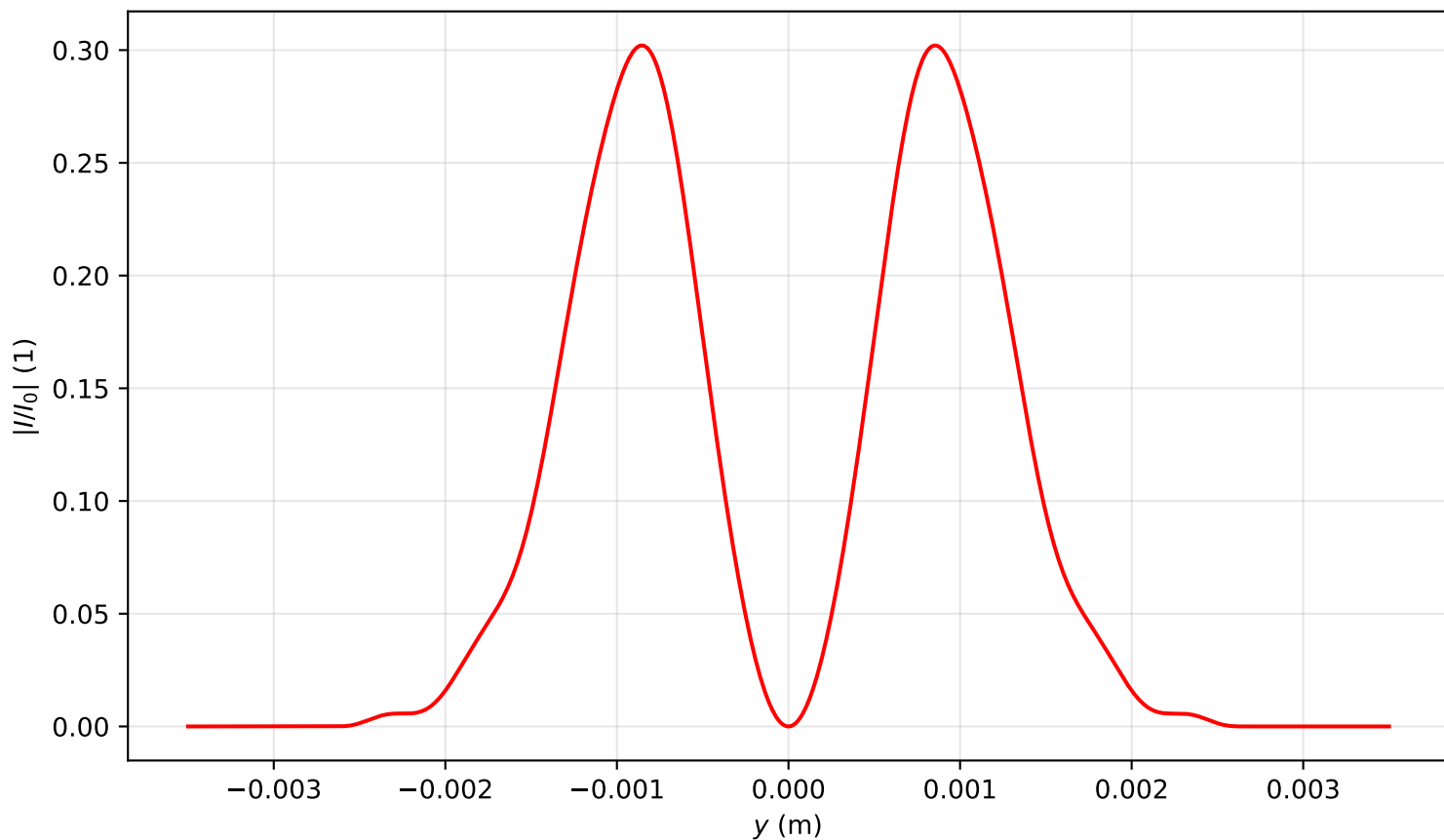
Intensity profile I(x=0, y, z=3.344)/I_0 , \text{Pin}=2.0\text{Pcr} , artificial time
